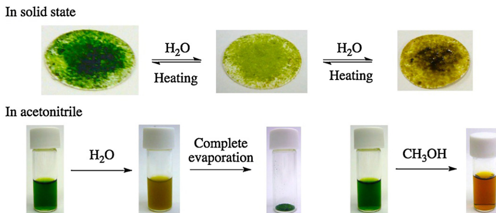
Fig. 9. The cobalt complex, [\text{Co}_2(\text{H}_2\text{O})_2\text{V}_{10}\text{O}_{30}]^{6-} , shows chromism between green and brown. It is deep green when dry and brown when moist. After exposure to water vapor, the color is restored by heating the sample. In acetonitrile solution, complete evaporation is necessary to restore the original color. The addition of alcohol also results in a brown color.
