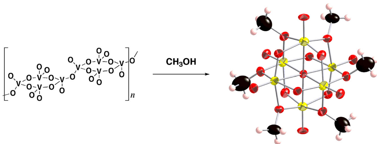
Fig. 6. The reaction pathway to the alkoxohexavanadate. The coordinatively unsaturated 1D (\text{PPh}_4)_2[\text{V}_4\text{O}_{11}] undergoes facile alcoholysis to give symmetrically substituted hexamethoxy-hexavanadate. Yellow, red, and black octants are vanadium, oxygen and carbon atoms, respectively.
