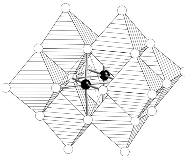
Fig. 4. Polyhedral representation of the disubstituted decavanadate structure. The shaded octahedra show \text{VO}_6 units. The filled circles represent the substituted heteroatoms at the central junction. The open circles represent oxygen atoms.
