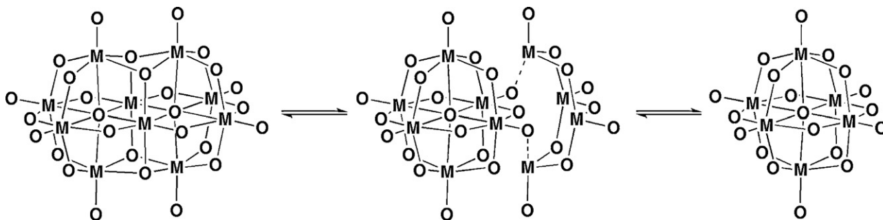
Fig. 5. Hypothetical mechanism of decametalate transformation. The base-promoted dissociation of the tetrameric fragment may lead to the formation of a hexametalate unit.
