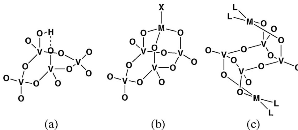
Fig. 2. The three representative coordination modes of the cyclic tetravanadate.
