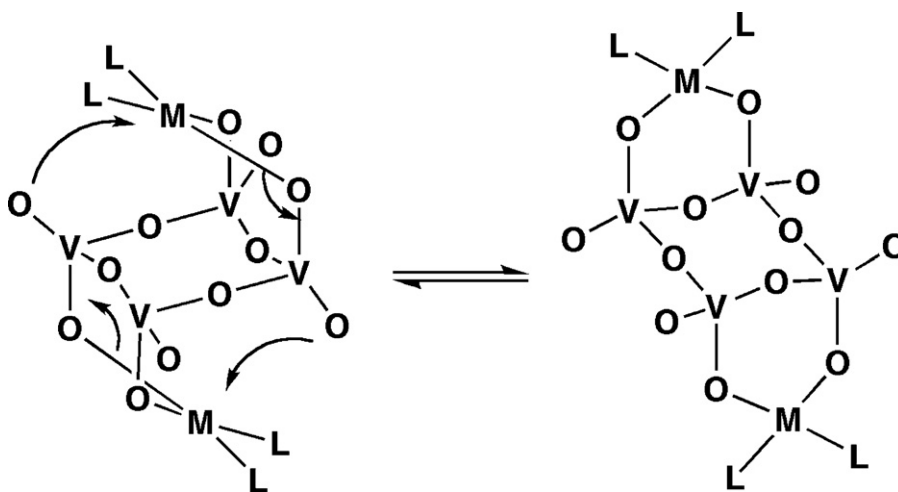
Fig. 3. The concerted pivoting mechanism of the tetravanadate-supported organometallic complexes.
