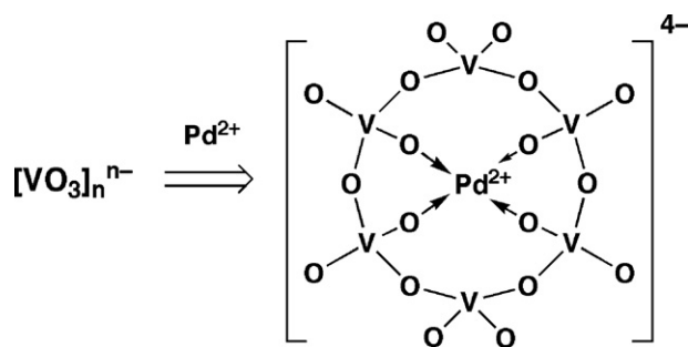
Fig. 7. The reaction scheme for the formation of a palladium complex. The template effect of a metal cation expands the ring size of the tetravanadate to form a disk-shaped all-inorganic coordination complex.
