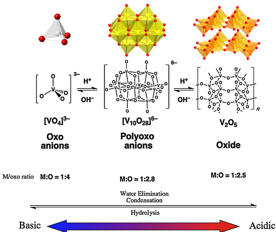
Fig. 1. The formal hydrolysis sequence of anions and oxides in vanadium (V) chemistry. Even in an extremely acidic medium, the hypothetical [\text{V}(\text{OH}_2)_6]^{5+} species is not observed. The main species observed under strong acidic conditions is cis -dioxo [\text{VO}_2(\text{OH}_2)_4]^+ .
