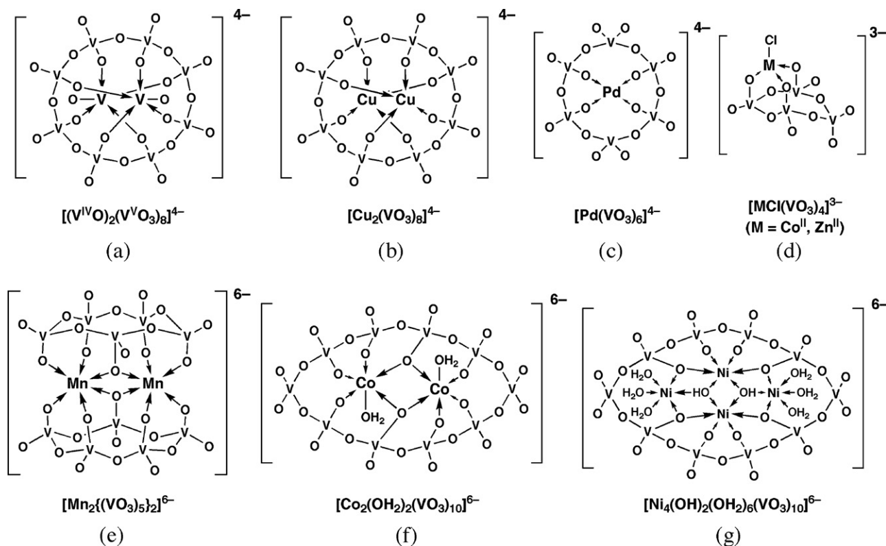
Fig. 8. The various all-inorganic macrocyclic complexes as heteropolyoxovanadates.
