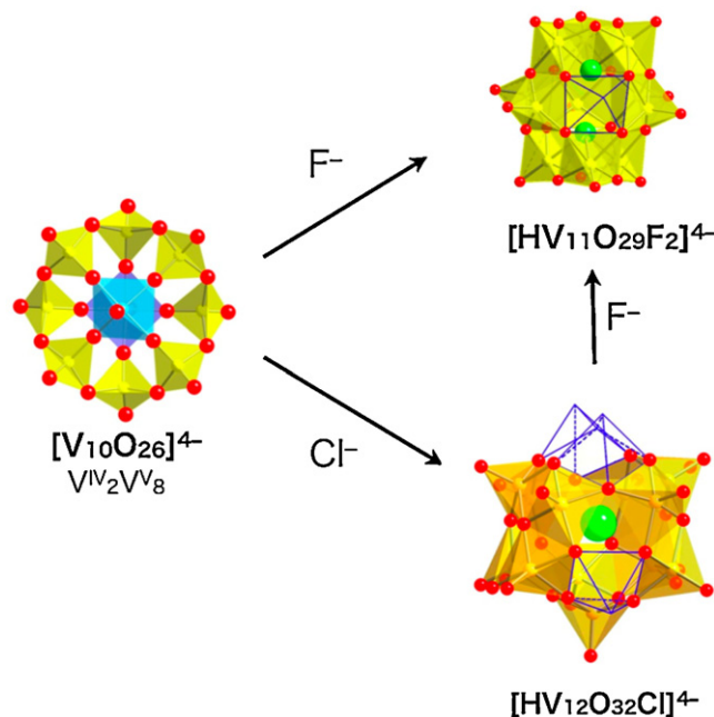
Fig. 10. Synthesis of lacunary polyoxovanadates from the reduced decavanadate: [\text{HV}^{\text{V}}_{11}\text{O}_{29}\text{F}_2]^{4-} and [\text{HV}_{12}\text{O}_{32}\text{Cl}]^{4-} . The yellow tetrahedra represent \text{VO}_4 units. The blue frames of empty pyramids represent the lacunary units.
