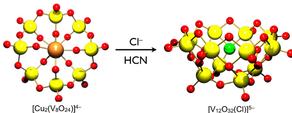
Fig. 11. Template switching reaction from a cation to an anion template for bowl type polyoxovanadate synthesis.
